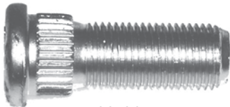
560-034 1/2-20R x 1-1/2" Knurl diameter: .618 (Code: F)
