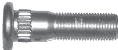
560-468 9/16-18R x 2-1/8" Knurl diameter: .650 (Code:KR)
