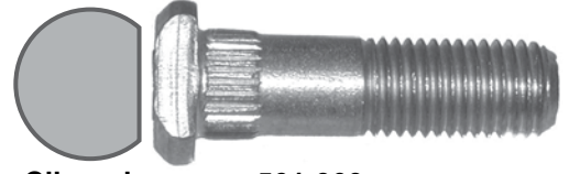
Clipped Head 561-309 M12 x 1.5 x 42.7mm Knurl diameter: 13.08mm
