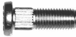
561-380 M10 X 1.25 x 29mm Knurl diameter: 10.0mm (Code: CS)
