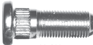
560-163 1/2-20R x 1-1/2" Knurl diameter: .545 (Code: BT)
