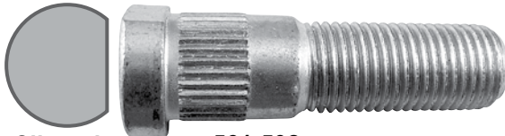
Clipped Head 561-502 M14 x 1.5 x 50mm Knurl diameter: 16.02mm
