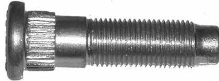
560-358 1/2-20R x 2" Knurl diameter: .612
