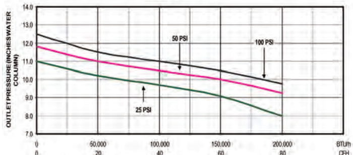
FLOW CHARACTERISTIC CHART FOR MODEL GR-700B
