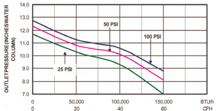
FLOW CHARACTERISTIC CHART FOR MODEL GR-700
