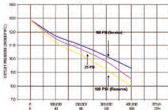
FLOW CHARACTERISTIC CHART FOR MODEL GR-9984-A
