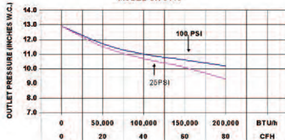
FLOW CHARACTERISTIC CHART FOR MODEL GR-9448
