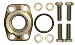
FLANGE PAD KIT Code 61 Female Pipe
