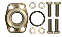
FLANGE PAD KIT Code 61 Female O-Ring
