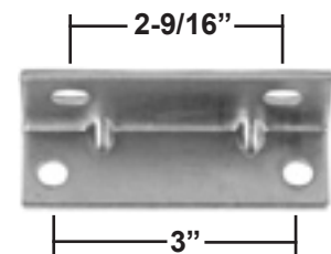
FS294314N "Standard"
