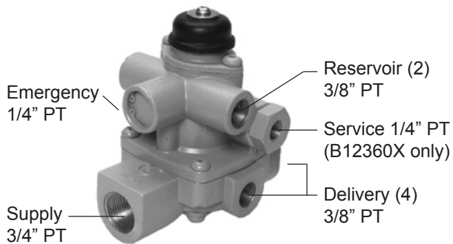
(B12360X Shown)
