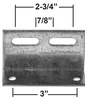
FS296010N "Universal"
