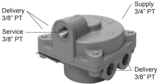
(B12343X Shown)
